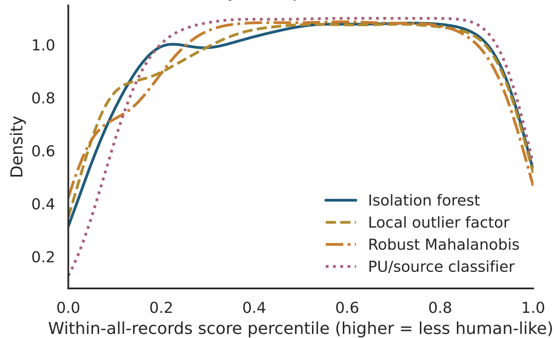
4581 anomaly-score percentile distributions
